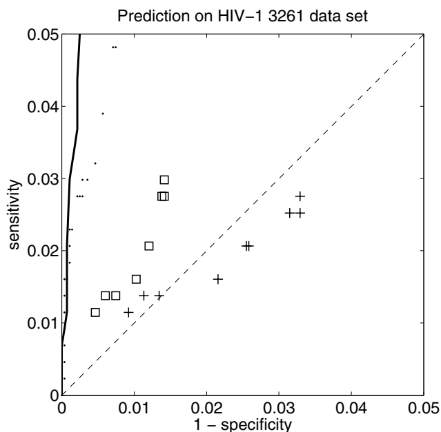
Figure 4 ROC for different rule based systems on the out-of-sample HIV-1 PR 3261 - detail. Detail of the receiver operator characteristic (ROC) for the OSRE rules' accuracy on the out-of-sample HIV-1 PR 3261 data set. The squares and the crosses are the results for Table 4 and Fig. 1a in [17]. The squares show the results when using 1, 2, 3, ..., and 10 rules from Fig. 1a in [17] and the crosses for Table 4 in [17]. The dots show the prediction accuracy for the HIVcleave web-server [37]. The solid curve shows the ROC curve for the hitherto best predictor, a linear support vector machine trained on the HIV-1 PR 1625 data set [38], which does not provide any rules. The dashed diagonal line marks the expected results for random prediction.
